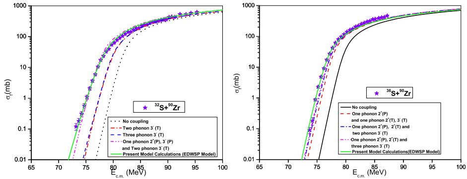
Fig. 2. The fusion excitation functions of ^{32,36}\text{S}+^{90}\text{Zr} systems obtained by using the EDWSP model and the coupled channel code CCFULL. The results are compared with available experimental data (*) taken from Ref. [30, 31].
