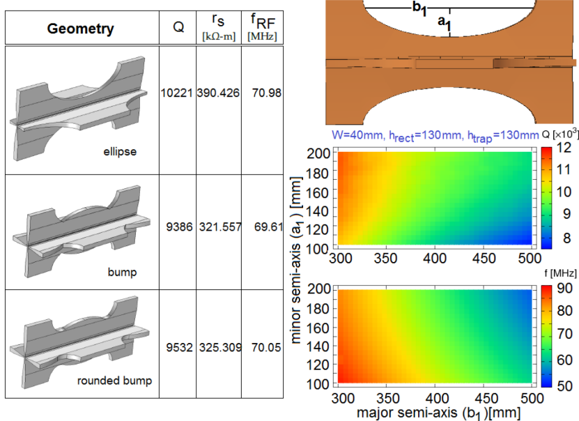
Fig. 3. Left: Three different shapes of the RF window considered in this study. Right: Evaluation of the quality factor Q and resonance frequency f as a function of semi-axes length a_1 and b_1 of the elliptical shapes.
