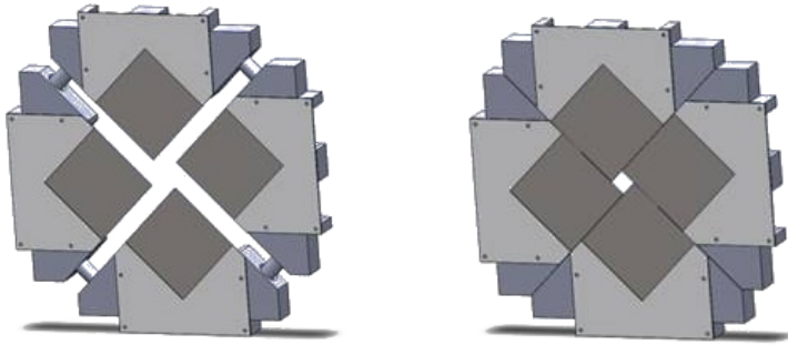
Fig. 1. Schematic layout of the in-ring Si detector array mounted on a 4-jaw actuator. The left figure shows the configuration when the beam is injected, the right figure when the beam is cooled.
