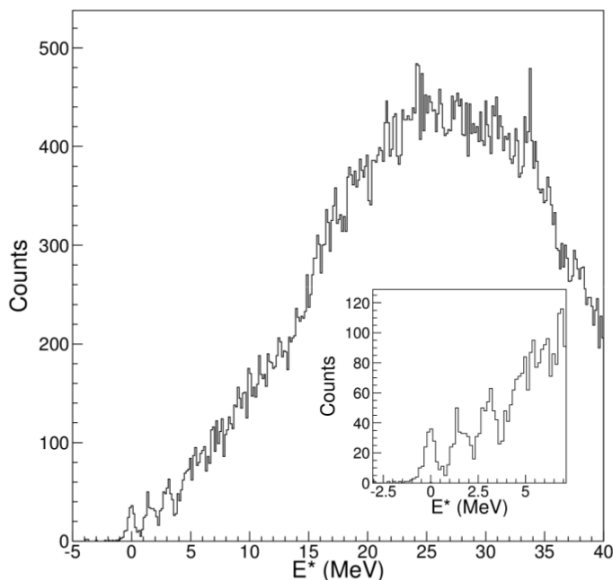
Fig. 1. Excitation energy spectrum of ^{40}\text{Ar} populated by the ^{40}\text{Ca}(^{18}\text{O}, ^{18}\text{Ne})^{40}\text{Ar} DCE reaction at 270 MeV. In the insert, a zoomed view of the low excitation energy region is shown.
