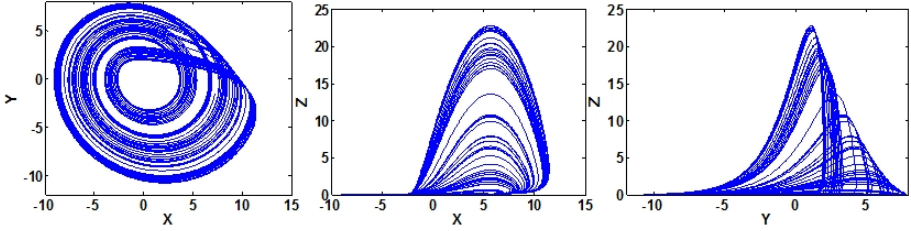
Fig. 1. (Color online) Rössler attractor from system (1) with a = b = 0.2 , c = 5.7 and initial conditions (x_0, y_0, z_0) = (-9, 0, 0) .
