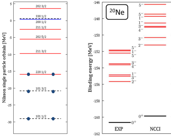
Fig. 1. (Color online) Left part shows a subset of neutron s.p. levels in the g.s. of ^{20}\text{Ne} relevant for this work. The orbitals are labelled with approximate Nilsson quantum numbers. Dots indicate occupied levels. Right part shows the calculated spectrum of negative-parity states in ^{20}\text{Ne} in absolute energy scale. See the text for further details.
