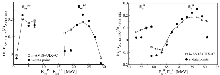
Fig. 1. Net effects of the Coulomb force in the cross section of the dp breakup at 130 MeV presented as a function of four invariants: E_{\text{rel}}^{pp} and E_{\text{rel}}^{pn} (left panel) and E_{\text{tr}}^p and E_{\text{tr}}^n (right panel). The coordinates represent the difference between the data and the results of Coulomb-less AV18+UIX calculations (dots) and the predicted Coulomb effect, i.e. the difference between both of the calculations AV18+UIX+C and AV18+UIX (empty squares).
