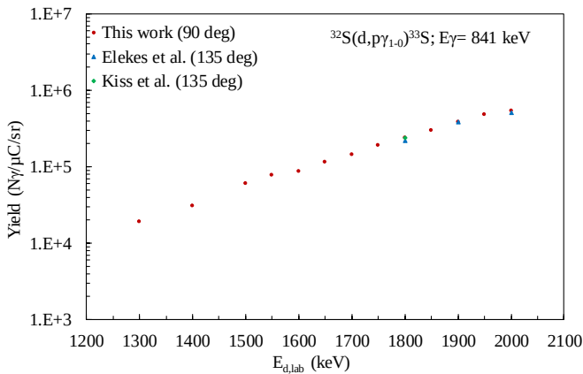
Fig. 6. The measured thick target yield data for the induced 841 keV gamma-ray emission due to ^{32}\text{S}(d, p\gamma_1)^{33}\text{S} reaction. For comparison, available data from the literature are also shown.
