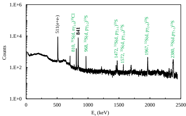
Fig. 5. The measured gamma-ray spectrum induced by 2000 keV deuterons from the thick Au/S target at 90^\circ .
