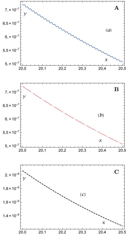
Fig. 2. Decay curves obtained for \omega_{\text{BW}}(m) given by Eq. (14). Axes: x = t/\tau_0 and y — survival probabilities: (a) the decay curve \mathcal{P}_p(t) , (b) the decay curve \mathcal{P}_0(t/\gamma) , (c) the decay curve \mathcal{P}_0(t) .
