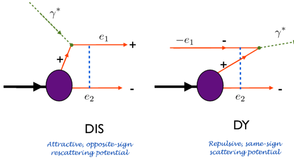
Fig. 18. Illustration of the Siverts effect from the initial-state versus the final-state interaction in DY and DIS reactions [100].
