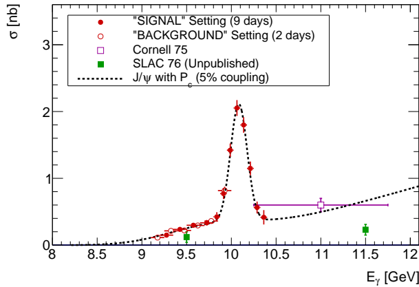
Fig. 23. Projected impact of this experiment assuming, the (5/2+, 3/2-) case with 5% coupling, for 9 days of data taking in setting No. 1 (solid circles) and 2 additional days of data taking in setting No. 2 (open circles). The existing data points from Cornell and SLAC (unpublished) are also shown.
