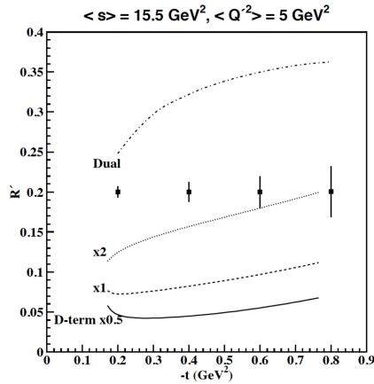
Fig. 17. Expected results from CLAS12 ( e^+e^- ) quasi-real photo-production measurements on the \cos(\phi_{\text{cm}}) moment of lepton decay angular distribution in one time-like photon kinematic bin as a function of transferred momentum squared, shown together with predictions of the dual parametrization model [88, 89] and double-distribution model [90] with different weights applied to the D -term contribution.
