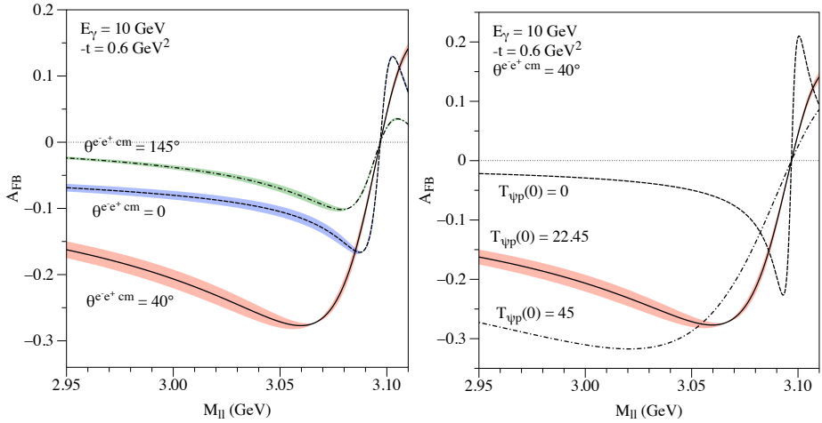
Fig. 10. Forward-backward asymmetry for the \gamma p \rightarrow e^- e^+ p process as a function of the dilepton mass M_{ll} around the \psi resonance: subtraction constant value T_{\psi p}(0) = 22.45 (left panel), and \theta_{\text{cm}}^{e^- e^+} = 40^\circ (right panel) [81].
