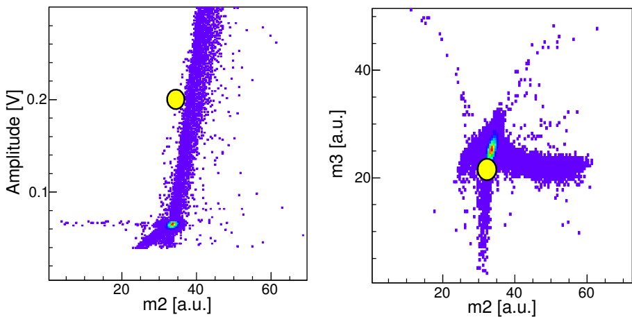
Fig. 3. (Colour on-line) Left: map of charge pulse amplitude versus m_2 of current pulse. Right: map of m_3 versus m_2 of current pulse. Measurement for Cf source.
