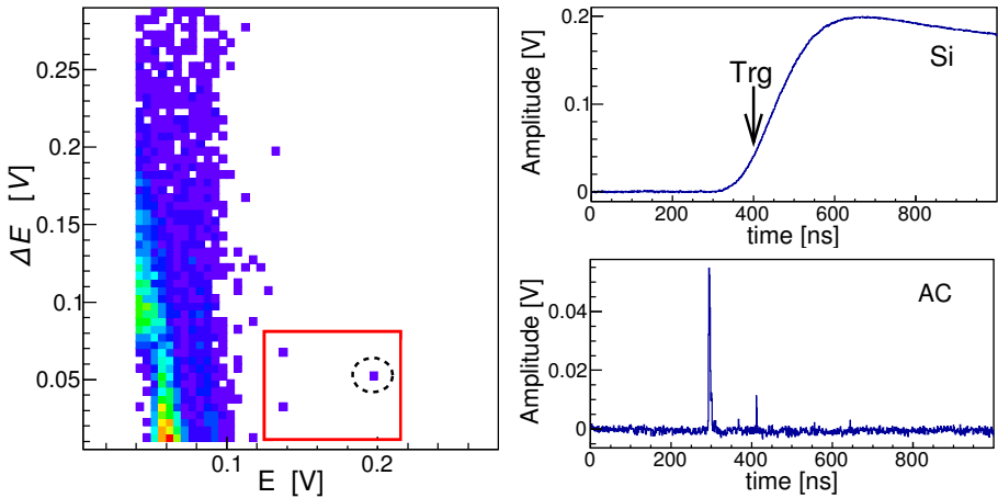
Fig. 2. Left: \Delta E - E coincidence signals map. Right: Signals from Si and AC detectors for the event marked inside dashed circle on the left panel.
