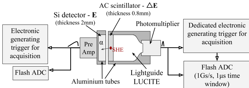
Fig. 1. Scheme of \Delta E - E detector. See the text for details.
