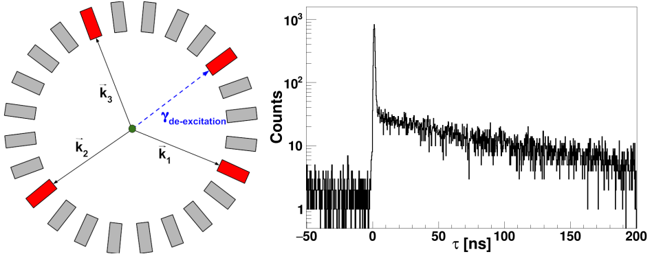
Fig. 1. Left panel: Scheme of the J-PET scanner registering signal candidates, de-excitation photon( \gamma_{\text{de-excitation}} ) represented using dashed blue line and three primary annihilation photons ( |\vec{k}_1| > |\vec{k}_2| > |\vec{k}_3| ). Right panel: positronium lifetime ( \tau ) distribution in the XAD-4 porous polymer, obtained from the measurement with the J-PET detector. The lifetime distribution is obtained by identifying and time stamping the de-excitation photon and the corresponding three annihilation photons from the decay of ortho-positronium.
