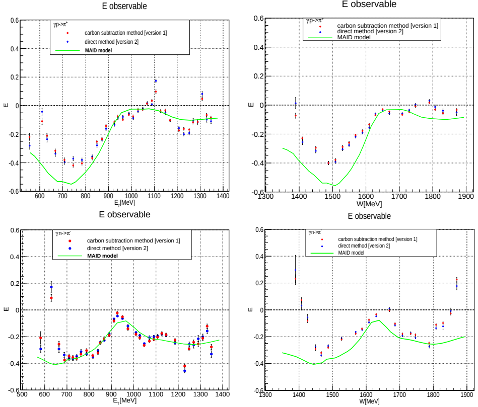
Fig. 2. (Color online) E -observable plots in terms of E_\gamma (photon energy) and W (center-of-mass energy) for \gamma p \rightarrow \pi^0 \pi^+ n (above row) and for \gamma n \rightarrow \pi^0 \pi^- p (bottom row); gray/red dots are for the method with carbon subtraction and the dark gray/blue dots correspond to the direct method; the gray/green line shape corresponds to that of predicted by MAID model.
