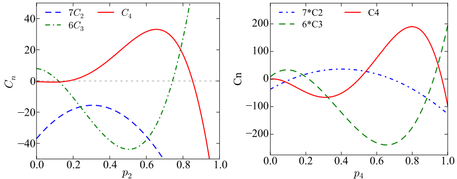
Fig. 2. Integrated multi-particle correlations C_n in the model where particles are correlated in pairs (left) and quartets (right) as a function of the probability for a pair ( p_2 ) or a quartet ( p_4 ) to end up in the rapidity bin. For larger values of p_2 and p_4 , we obtain large values of C_3 and C_4 . See the text for further explanation.
