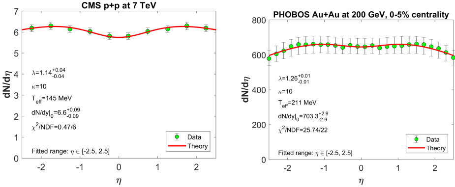
Fig. 3. Left panel shows fits with the CKCJ hydro-solution to CMS p+p data at \sqrt{s} = 7 TeV, using T_{\text{eff}} = 145 MeV. The right panel is the same, but for PHOBOS Au+Au data at \sqrt{s_{NN}} = 200 GeV in the 0-5% centrality class, using T_{\text{eff}} = 211 MeV. The speed of sound is fixed to c_s^2 = 1/\kappa = 0.1 in both cases.
