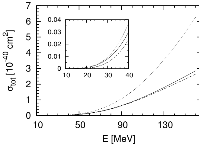
Fig. 2. The total breakup cross section for inclusive charged-current electron antineutrino disintegration of ^3\text{H} (dashed line), neutral-current electron antineutrino disintegration of ^3\text{H} (solid line), and neutral-current electron neutrino disintegration of ^3\text{H} (dotted line) as a function of the laboratory (anti)neutrino energy E . The figure was originally published in [52].
