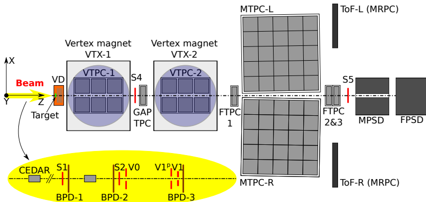
Fig. 1. NA61/SHINE detector subsystems after LS2 upgrade.
