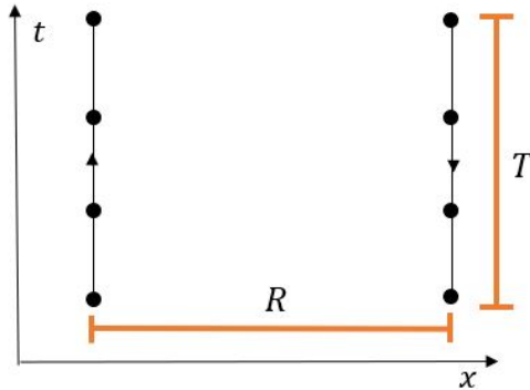
Fig. 2. Time-like Wilson lines L(T, \vec{0}) and L(T, \vec{r})^\dagger on the lattice.
