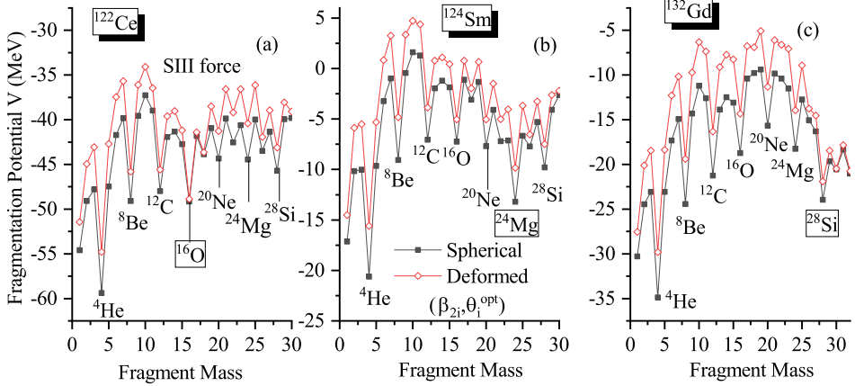
Fig. 1. PCM calculated fragmentation potentials for the decay of (a) ^{122}\text{Ce} , (b) ^{124}\text{Sm} , and (c) ^{132}\text{Gd} considering spherical and \beta_2 deformed choice of decay-fragments.
