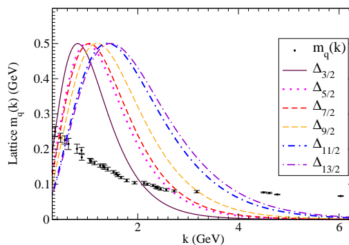
Fig. 2. Typical momentum distributions of increasingly excited \Delta_{3/2}, \dots, \Delta_{13/2} resonances overlap less and less with the dynamically generated IR quark mass so that \langle n | (m(k)/k) H_\chi^{\text{QCD}'} | n \rangle becomes small. (Illustrative variational wavefunctions for a linear potential with string tension \sigma = 0.135 \text{ GeV}^2 , not normalized for visibility.) This computation has been reported in [6].
