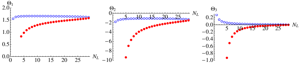
Fig. 6. Critical exponents for the NGFPs in the leading order truncation as a function of N_L . The fixed point corresponding to the open circles has two relevant directions, whereas the fixed point corresponding to the filled circles has only one relevant direction.
