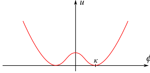
Fig. 3. Sketch of the scale-dependent effective potential u as a function of the field \phi_a . For a theory in the regime of spontaneously broken symmetry we employ an expansion about a positive minimum at \kappa , corresponding to a nonvanishing vacuum expectation value (v.e.v.) for the bosonic field.
