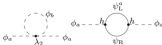
Fig. 5. Loop contributions to the renormalization flow of the Higgs dimensionless vev. The loop on the l.h.s. couples all available boson components giving a linear dependence on N_L . This is not the case for the fermionic loop on the r.h.s. which is fully determined by the incoming boson field component.
