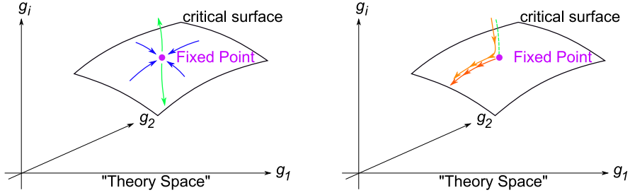
Fig. 2. Left panel: flow towards the UV in the vicinity of the fixed point. Relevant directions approach the fixed point (dark gray/blue arrows) and span the critical surface; irrelevant directions run away from the fixed point for k \rightarrow \infty (light gray/green arrows). Right panel: flow towards the IR. As the irrelevant directions are strongly attracted to the critical surface, the IR observables of the theory are solely determined by the relevant directions.
