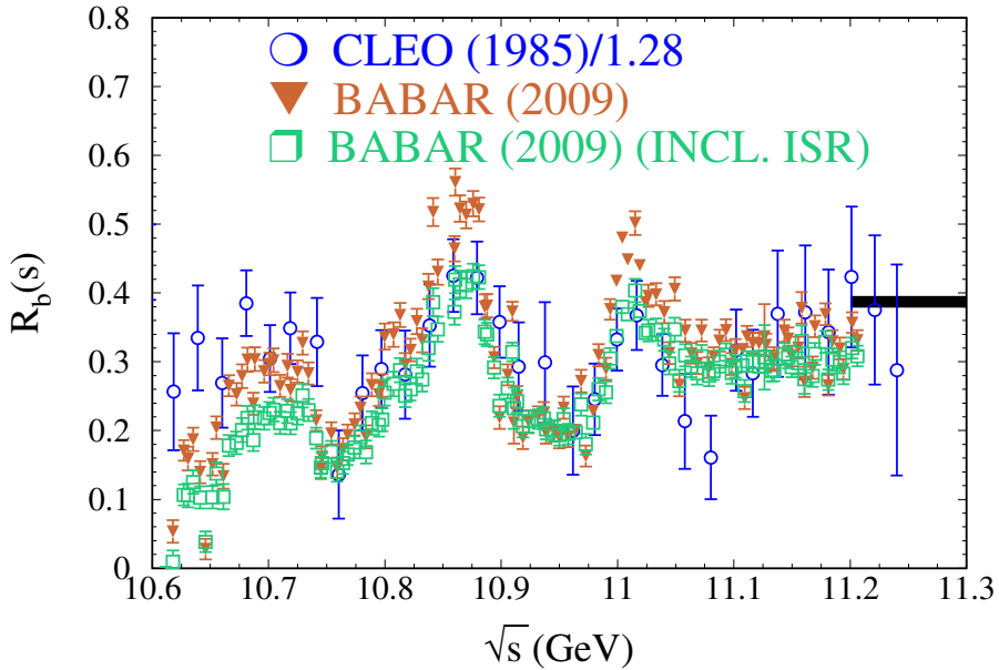
Fig. 1. Comparison of rescaled CLEO data for R_b with BaBar data before and after deconvolution. The black bar on the right corresponds to the theory prediction [20].
