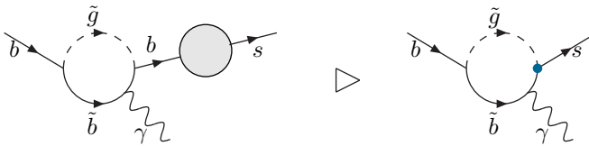
Fig. 2. Gluino diagram giving a contribution to b \rightarrow s\gamma of the form (\text{loop} \times \tan\beta)^2 . Left: External leg method. Right: Effective vertex method.
