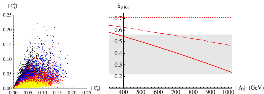
Fig. 3. Left: Magnitudes of chargino and gluino contributions to C_8 scanned over the MSSM parameter space. Right: S_{\phi K_S} as a function of |A_t| .
