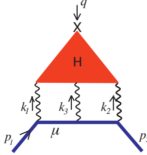
Fig. 2. Hadronic light-by-light contribution to a_\mu .
