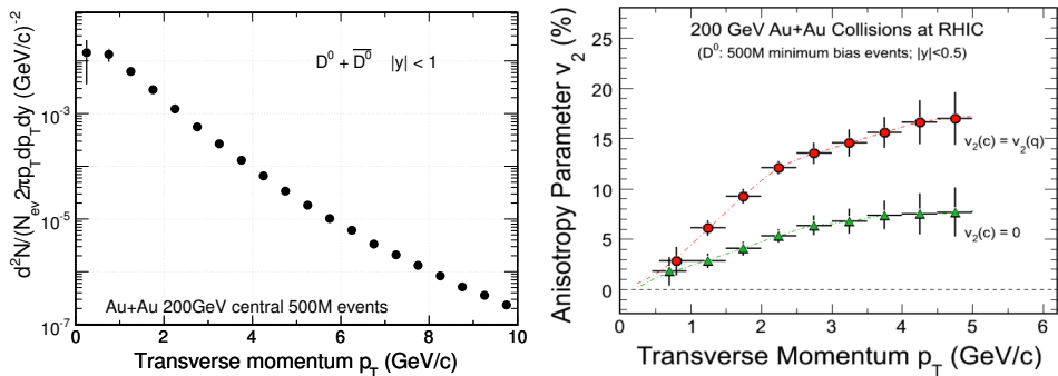
Fig. 1. Projections of key measurements with HFT. The left panel shows the anticipated first year (or a sample of 500 million events) p_T spectra of D^0 s. The right panel shows the anticipated accuracy in determining the D^0 elliptic flow. The error bars shown in both plots are based on S/N estimates for this event sample.
