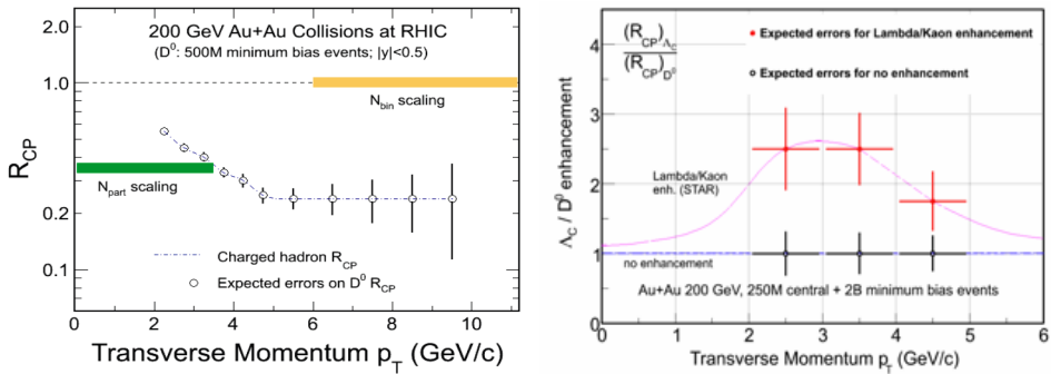
Fig. 2. (Left panel) Expected errors for the R_{CP} measurement as a function of p_T . (Right panel) Statistical errors of the \Lambda_C/D^0 ratio for the case of no enhancement and of \Lambda/K_S^0 -like enhancement.
