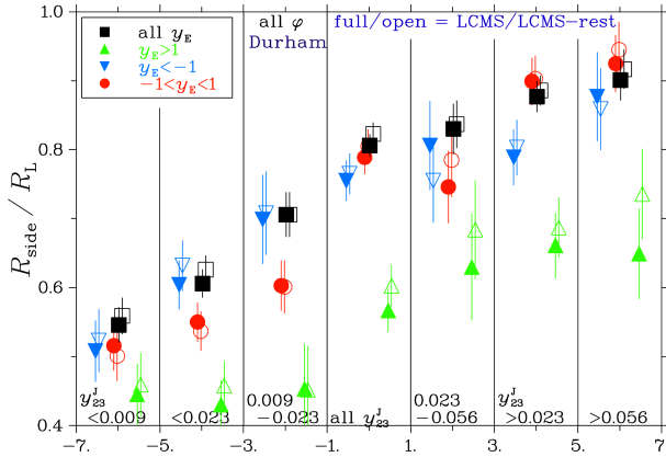
Fig. 4. Values of the ratio of the radii, R_{\text{side}}/R_L , from fits of Eq. (6) with Eqs. (5) and (7) for various y_{23} subsamples with selections on the rapidity, y_E , of the pair.
