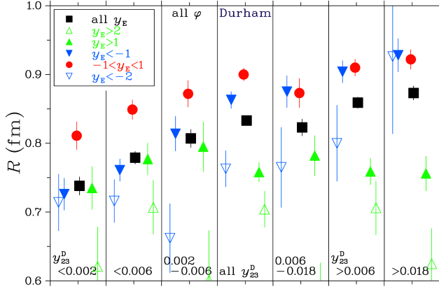
Fig. 2. Values of the effective radius, R , from fits of Eq. (1) for various y_{23}^D subsamples with selections on the rapidity, y_E , of the pair.
