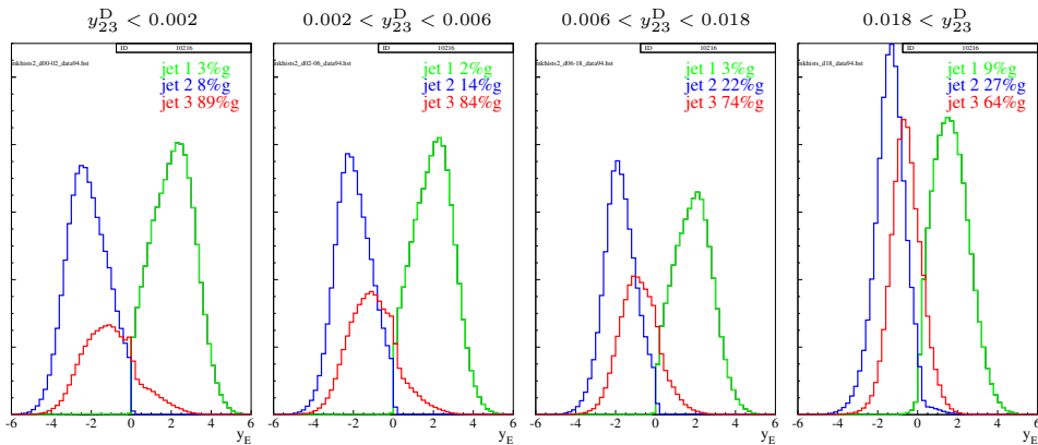
Fig. 1. Rapidity, y_E , distributions of particles from jets 1, 2, and 3 for various y_{23}^D subsamples.
