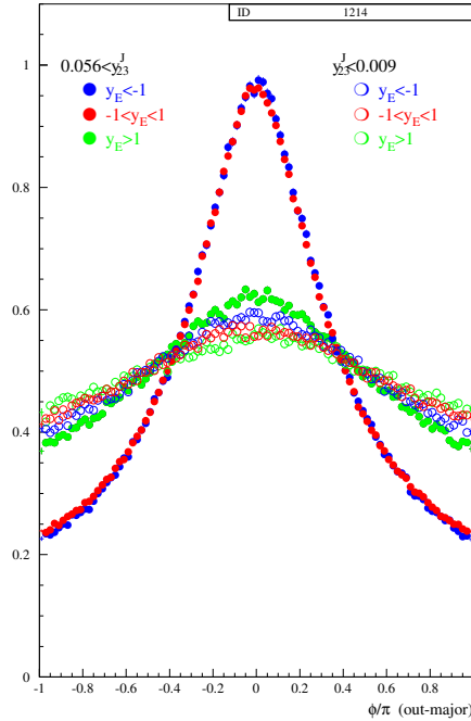
Fig. 5. The azimuthal angle of the out direction with respect to the major direction for well-separated three-jet events and for narrow two-jet events for three intervals of pair rapidity, y_E .
