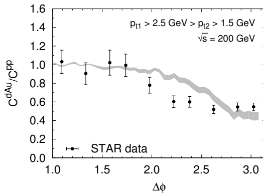
Fig. 2. Ratio of d -Au/ p - p coincidence probabilities C(\Delta\phi) for the forward dihadron production at RHIC as a function of the azimuthal distance between the particles. The band corresponds to our prediction with the uncertainty related to unknown yield of uncorrelated dihadron production. For full details, see [8].
