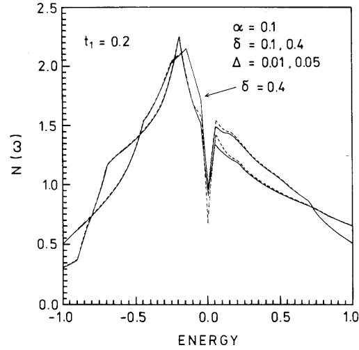
Fig. 4. Same as in Fig. 2 in SC phase for values of \Delta = 10^{-2} , and 5 \times 10^{-2} , for \delta = 0.1 (full line) and \delta = 0.4 (dashed line).
