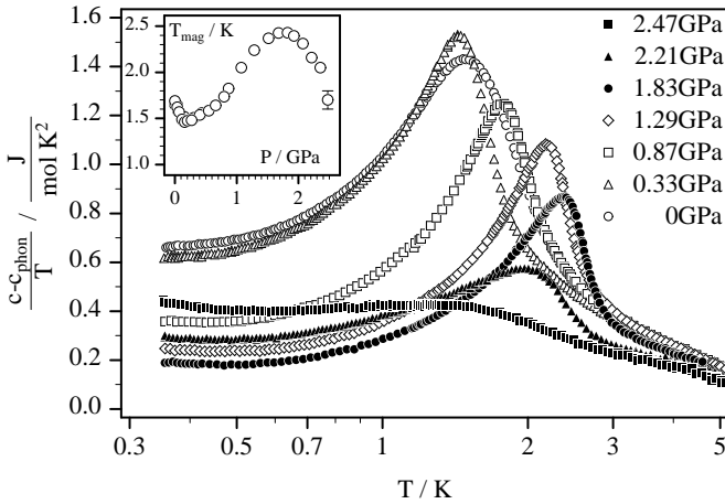
Fig. 1. Magnetic specific heat in a logarithmic scale. Insert: T_{\text{mag}} as defined by the position of the maximum in C(T) .
