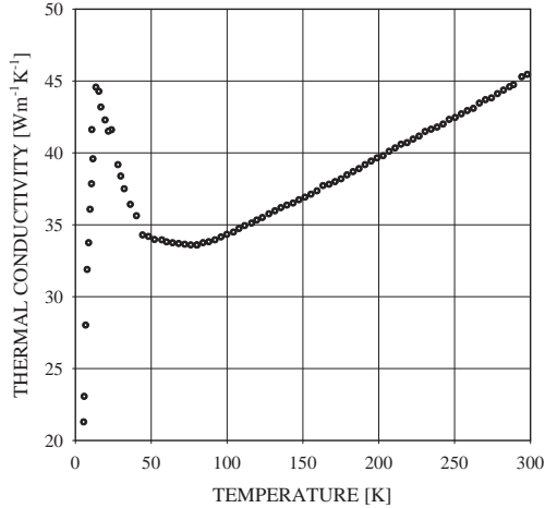
Fig. 1. Temperature dependence of the thermal conductivity for \text{LaSn}_3 .
