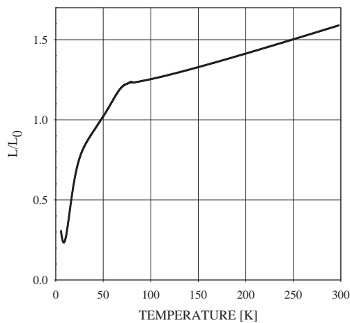
Fig. 2. Temperature dependence of the reduced Lorenz function for \text{LaSn}_3 .
