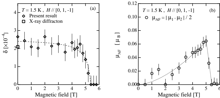
Fig. 2. Magnetic-field dependences of (a) displacement parameter \delta for the Fe-ion coordination and of (b) field-induced AF moment \mu_{\text{AF}} . Lines are guide to eyes.
