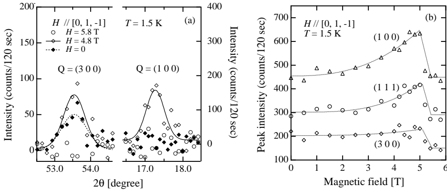
Fig. 1. (a) Scan profiles of superlattice reflections at \mathbf{Q} = (3, 0, 0) and (1, 0, 0) . The intensities are the difference between the measured counts at 1.5 K and those at 10.3 K in zero field. (b) Magnetic-field dependences of superlattice reflections at \mathbf{Q} = (1, 0, 0) , (1, 1, 1) and (3, 0, 0) at 1.5 K. Lines are guide to eyes.
