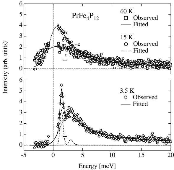
Fig. 1. Inelastic neutron scattering spectra of polycrystalline \text{PrFe}_4\text{P}_{12} .
