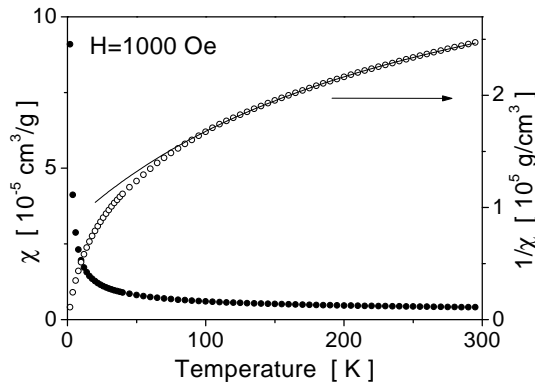
Fig. 1. Magnetic dc-susceptibility of CeRhSn in H = 1000 Oe. The solid line is the Curie–Weiss fit in the temperature range 120–300 K (see text).
