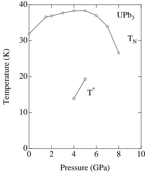
Fig. 2. Pressure phase diagram in UPb 3 .
