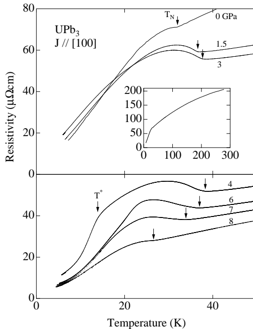
Fig. 1. Temperature dependence of the electrical resistivity under pressure in \text{UPb}_3 .
