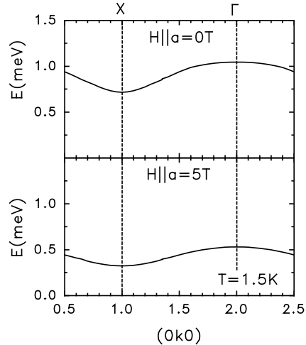
Fig. 4. Calculated dispersion curves with an isotropic exchange interaction in CeCu_2 in zero field and for a field of 5 T in a -direction. The lines are results of a calculation using the McPhase [7] program.
