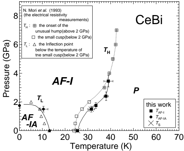
Fig. 2. The magnetic P - T phase diagram of CeBi.
