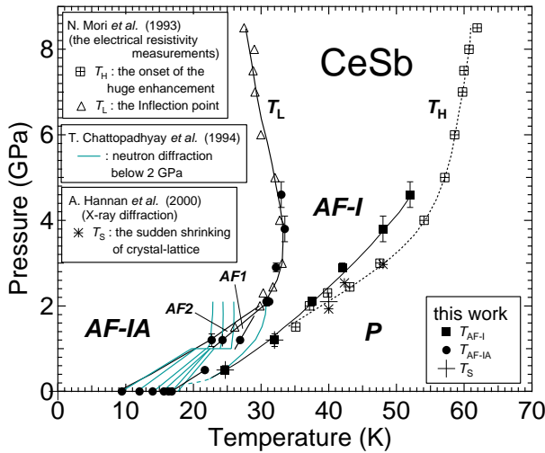
Fig. 1. The magnetic P - T phase diagram of CeSb .
