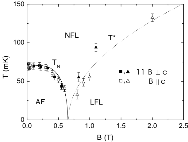
Fig. 5. T - B phase diagram for \text{YbRh}_2\text{Si}_2 with T_N as derived from d\rho/dT vs T and T^* , the upper limit of the \Delta\rho = AT^2 behavior, as a function of magnetic field, applied both along and perpendicular to the c -axis. For the latter ones the B -values have been multiplied by a factor 11. Lines separating the antiferromagnetic (AF), non-Fermi liquid (NFL) and Landau Fermi liquid (LFL) phase are guides to the eye.
