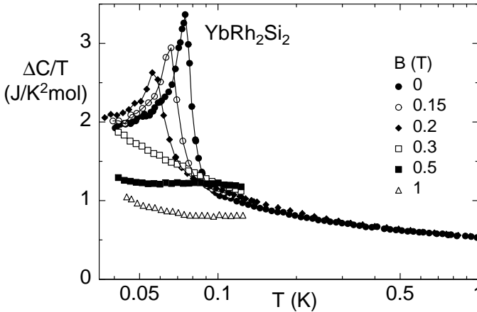
Fig. 6. Specific heat as \Delta C/T = (C - C_Q)/T vs T (on a logarithmic scale) for \text{YbRh}_2\text{Si}_2 at varying fields applied parallel to the c -axis. C_Q \sim T^{-2} is the nuclear quadrupole contribution calculated from recent Mössbauer results [14].
