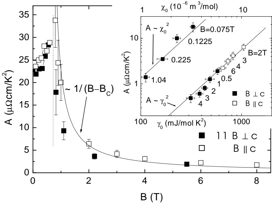
Fig. 7. Coefficient A = \Delta\rho/T^2 vs field B . Data for B perpendicular to the c -direction have been multiplied by 11. Dashed line marks B_{c0} , solid line represents (B - B_{c0})^{-1} . Inset shows double-log plot of A vs \gamma_0 and A vs \chi_0 for different magnetic fields. Solid lines represent A/\gamma_0^2 = 5.8 \times 10^{-6} \mu\Omega\text{cm}(\text{Kmol}/\text{mJ})^2 and A/\chi_0^2 = 1.25 \times 10^{12} \mu\Omega\text{cmK}^{-2}/(\text{m}^3/\text{mol})^2 .
