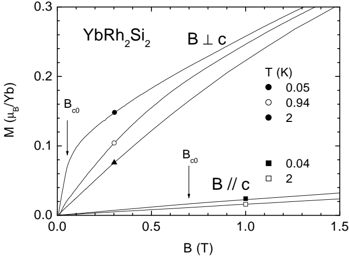
Fig. 3. Isothermal DC magnetization M at varying temperatures in magnetic fields applied along and perpendicular to the c -axis. Arrows indicate critical fields B_{c0} .
