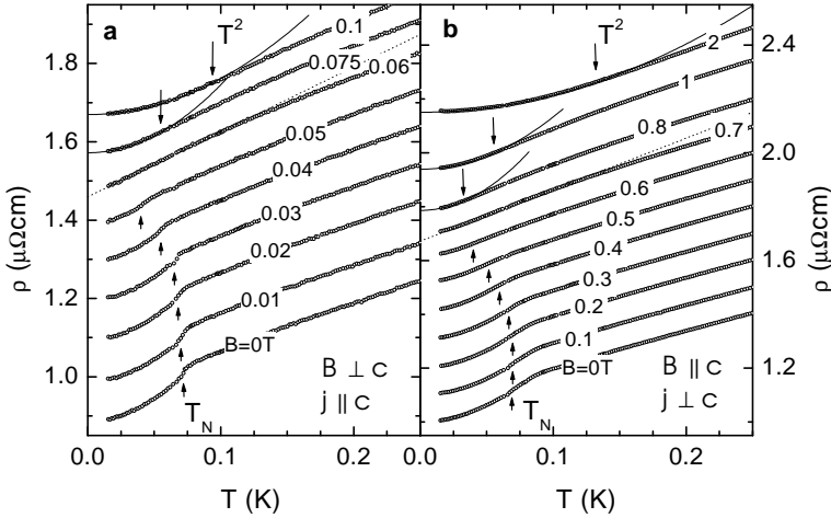
Fig. 4. Low-temperature electrical resistivity of \text{YbRh}_2\text{Si}_2 at varying magnetic fields applied perpendicular (a) and along the c -axis (b). For clarity the different curves in B > 0 were shifted subsequently by 0.1 \mu\Omega\text{cm} . Up- and down-raising arrows indicate T_N and upper limit of T^2 behavior, respectively. Dotted and solid lines represent \Delta\rho \sim T^\varepsilon with \varepsilon = 1 and \varepsilon = 2 , respectively.
