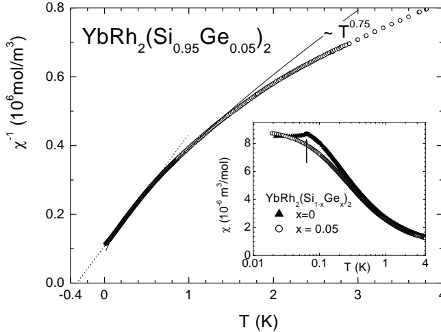
Fig. 2. Inverse of the AC-susceptibility in the easy-magnetic plane perpendicular to the crystallographic c -direction, as \chi^{-1} vs T for \text{YbRh}_2(\text{Si}_{0.95}\text{Ge}_{0.05})_2 . The dotted line indicates Curie–Weiss type dependence \chi(T) = C/(T - \theta) implying large fluctuating moments of 1.4 \mu_B/\text{Yb}^{3+} -ion and a Weiss temperature of \theta \simeq -0.3 \text{ K} . The solid line represents \chi^{-1} \sim T^\alpha with \alpha \approx 0.75 (see text). The inset shows \chi vs T on a logarithmic scale for \text{YbRh}_2(\text{Si}_{1-x}\text{Ge}_x)_2 for x = 0 and 0.05 . The arrow indicates T_N for the undoped system.
