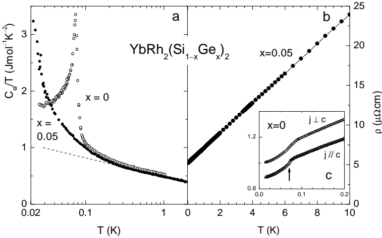
Fig. 1. Comparison of the low-temperature electronic specific heat C_{\text{el}} = C - C_Q as C_{\text{el}}/T vs \log(T) (a) and the electrical resistivity \rho (b and c) of high-quality \text{YbRh}_2(\text{Si}_{1-x}\text{Ge}_x)_2 single crystals with Ge-contents x = 0 and x = 0.05 . C_Q \sim T^{-2} is the nuclear quadrupole contribution calculated from recent Mössbauer results [14]. Dotted line in (a) marks \log(T_0/T) dependence with T_0 \simeq 24 \text{ K} . Resistivity data shown in (c) were obtained for the current \mathbf{j} flowing along ( \Delta ) and perpendicular ( \circ ) to the c -axis. The arrow indicates T_N as obtained from the maximum in d\rho/dT .
