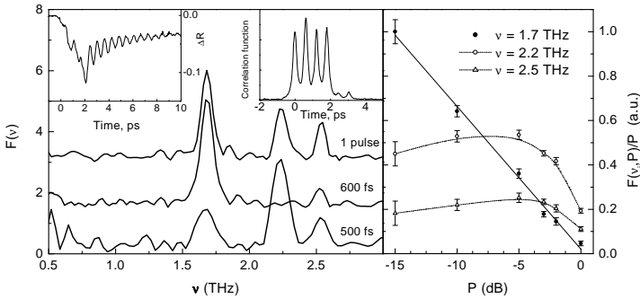
Fig. 2. Left panel: Fourier spectrum of the transient response for the single pulse excitation (A), and the four pulse trains for two different pulse separations. Left insert: transient reflectivity, induced by four-pulse trains. Right insert: cross-correlation of the pump pulse train with the probe. Right panel: Normalized pump-power dependence of the amplitudon (1.7 THz) and two Raman phonons (2.2 THz and 2.5 THz).
