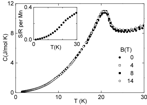
Fig. 1. Specific heat C as a function of temperature T of \text{Mn}_3\text{Si} . The anomaly corresponds with the ordering temperature at T_N \approx 23 K. The rounding may be attributed to the polycrystalline nature of the samples studied here. T_N is not affected by high magnetic field up to 14 T, apart from a slight increase of 3% above T_N .
