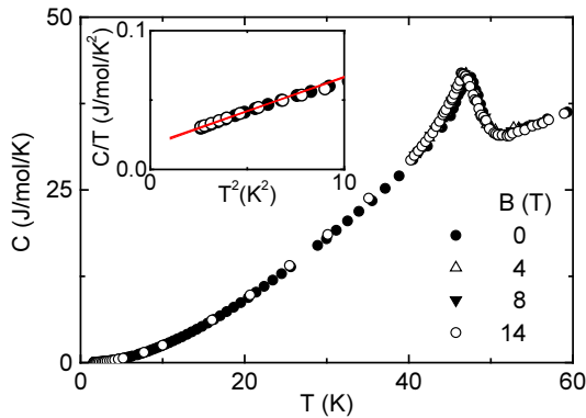
Fig. 2. Specific heat C as a function of temperature T of CuMnSb . The anomaly corresponds with the antiferromagnetic ordering temperature T_N \approx 50K . In small fields the transition becomes slightly sharper, probably due to the polycrystalline nature of the samples. At high magnetic field T_N remains unchanged.
