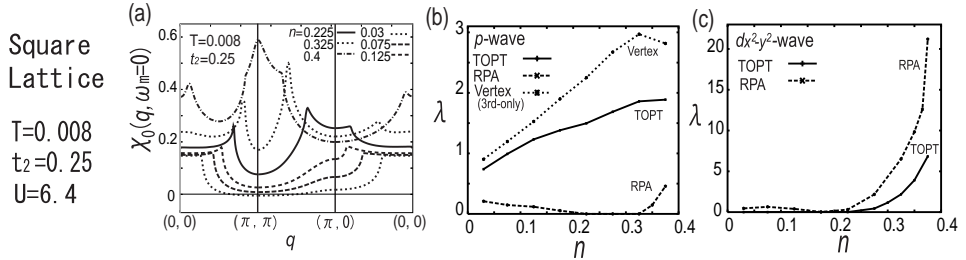
Fig. 2. (a) The dependence of the bare susceptibility \chi_0(\vec{q}, \omega_n = 0) on the density n in the square lattice. (b), (c) The dependence of the eigenvalue \lambda on the density n in the cases of the p - (b) and d_{x^2-y^2} (c) wave pairings in the square lattice.
