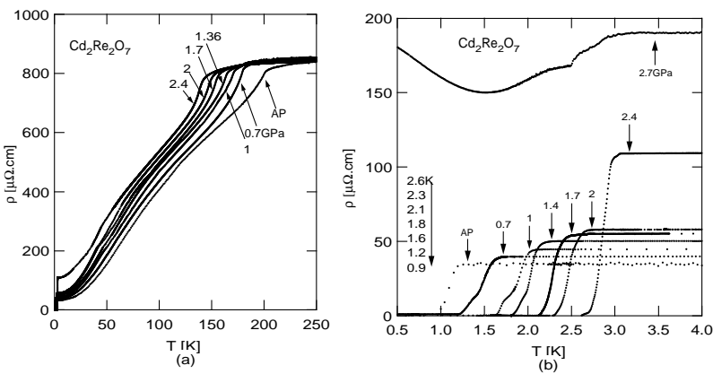
Fig. 1. Temperature dependence of resistivity of \text{Cd}_2\text{Re}_2\text{O}_7 for various pressure (a). Temperature dependence of resistivity of \text{Cd}_2\text{Re}_2\text{O}_7 in a low temperature region for various pressures (b).
