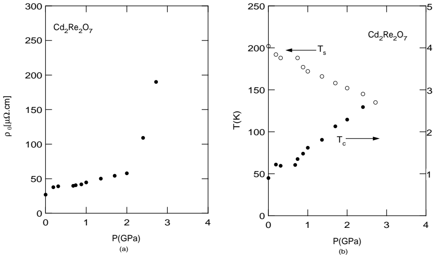
Fig. 2. Pressure dependence of residual resistivity of Cd_2Re_2O_7 (a), P - T phase diagram of Cd_2Re_2O_7 (b).
