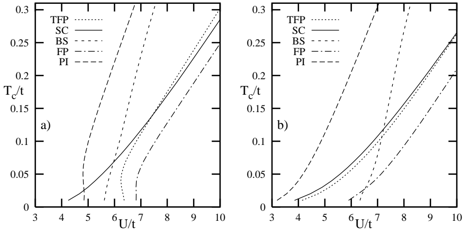
Fig. 1. Temperature phase diagram of the model at t' = -t/6 for n = 0.95 (a) and n = 0.86 (b). SC stands for superconductivity, BS for band splitting, PI for Pomeranchuk instability, FP for flux phase, and TFP for triplet flux phase.
