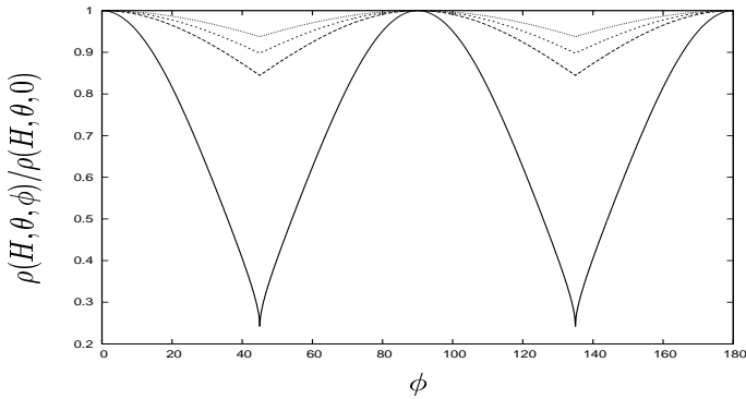
Fig. 2. The magnetoresistance is shown as a function of \phi for \theta = 90^\circ, 60^\circ, 45^\circ and 30^\circ from bottom to top.
