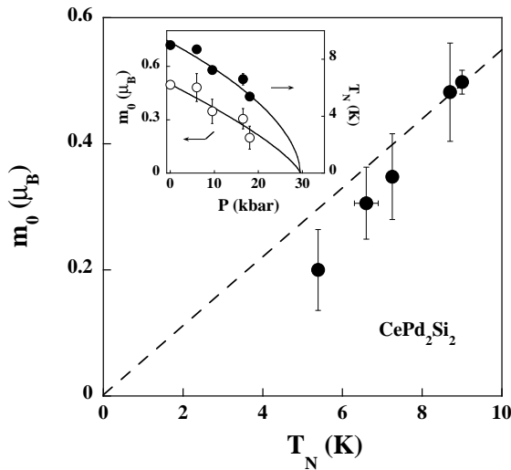
Fig. 2. Variation of the staggered magnetic moment m_0 with respect to the Néel temperature T_N . The inset shows the pressure variation of m_0 and T_N . Lines are guides for the eyes.
