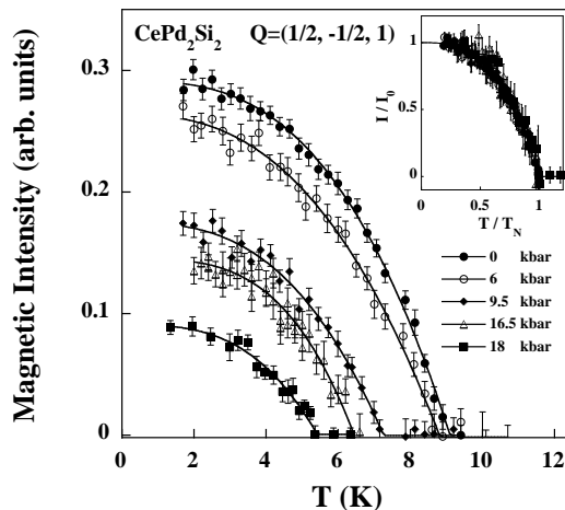
Fig. 1. Intensity of the magnetic (1/2, -1/2, 1) reflection as a function of temperature for several pressures. The inset shows the collapse of the same data plotted in reduced variables: I/I_0 as a function of T/T_N . Lines correspond to fit as indicated in the text.
