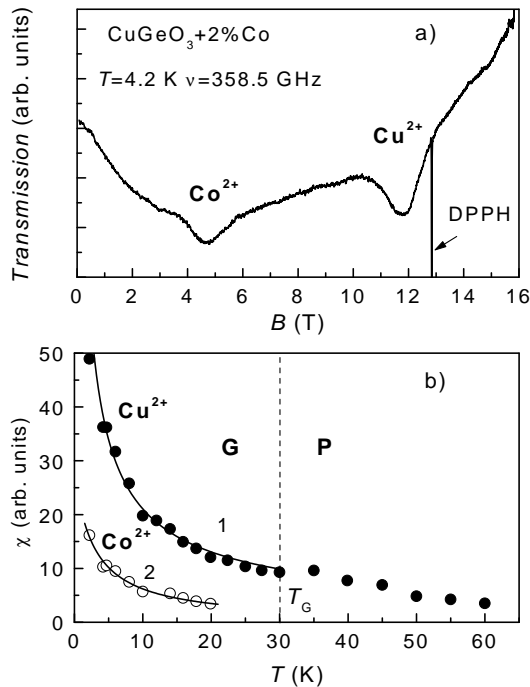
Fig. 1. (a) ESR spectrum for Co-doped sample in geometry B \parallel a . Arrow mark reference spectrum for DPPH. (b) \chi(T) data for \text{Cu}^{2+} chains and \text{Co}^{2+} impurity. 1- power law (1) with \alpha=0.69 , 2- Curie-Weiss law.
