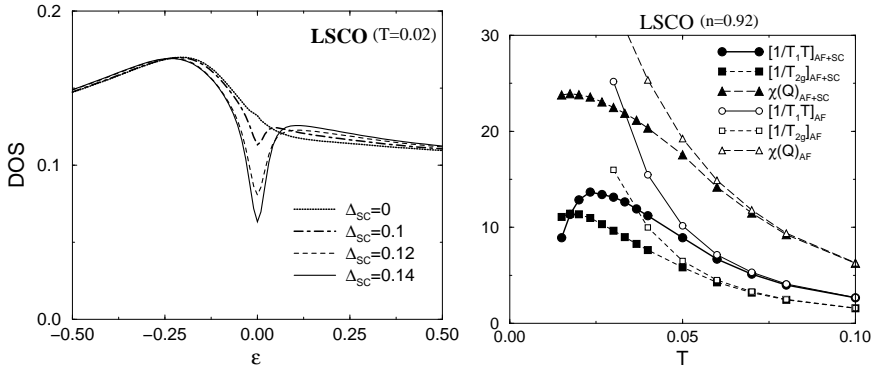
Fig. 1. DOS, \chi_Q , 1/T_1T and 1/T_{2g} studied by the FLEX+ T -matrix approximation (AF+SC). Results by the FLEX approximation (AF) is also shown. T = 0.1 corresponds to 500K.
