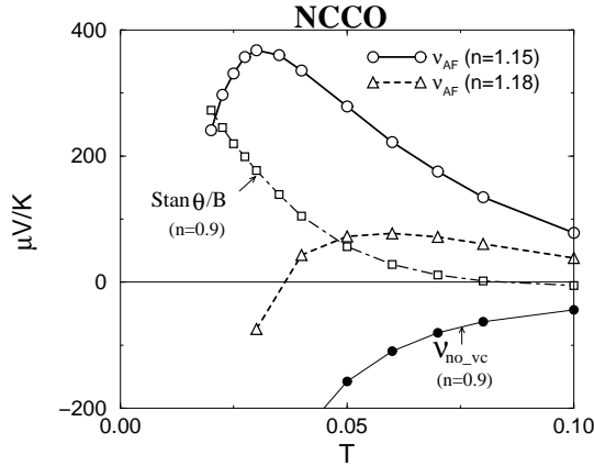
Fig. 3. \nu and S \tan \theta_H given by the FLEX approximation for NCCO
