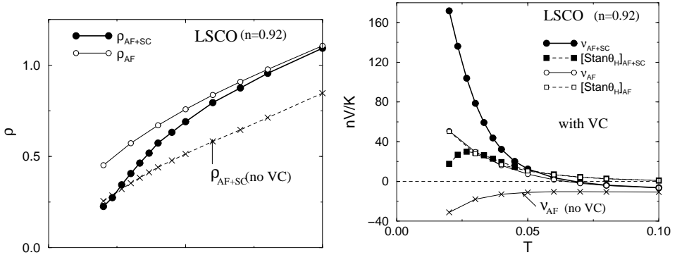
Fig. 2. \rho , \nu and S \tan \theta_H given by the FLEX+ T -matrix approximation (AF+SC) for LSCO.
