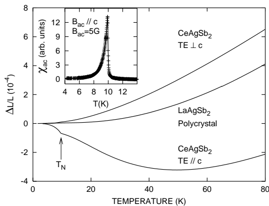
Fig. 1. Linear thermal expansion ( \Delta L/L ) versus temperature of \text{CeAgSb}_2 single crystal and \text{LaAgSb}_2 polycrystal. The inset shows temperature dependence of inductive, \chi'_{\text{ac}}(T) component of the ac-susceptibility for B_{\text{ac}} \parallel c .
