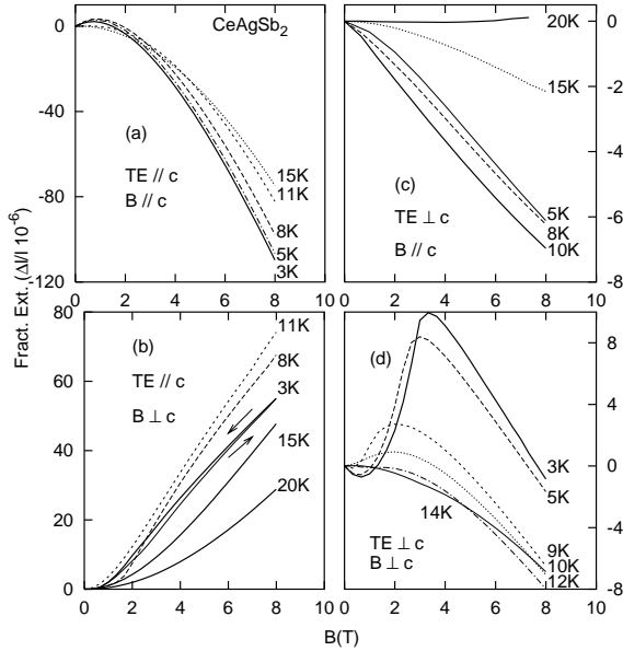
Fig. 3. The magnetostriction isotherms at various temperatures of CeAgSb_2 single crystal, (a) and (b) (\Delta L/L) \parallel c and, (c) and (d) (\Delta L/L) \perp c , for both B \parallel c and B \perp c .
