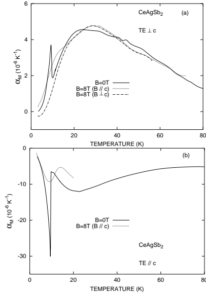
Fig. 2. The magnetic contribution to the linear thermal expansion coefficient, \alpha_M(T) of CeAgSb_2 single crystal in zero field and 8T field, (a) TE \perp c and, (b) TE \parallel c .
