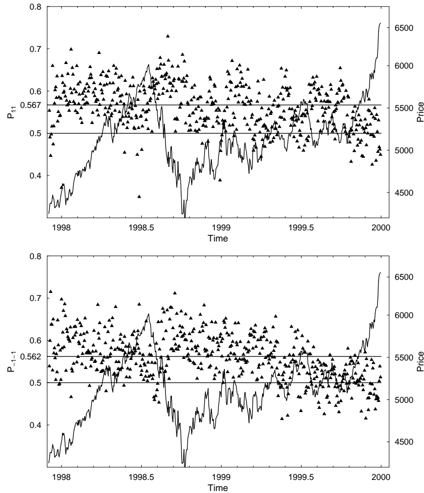
Fig. 1. The DAX time dependence over the period 01.12.1997–31.12.1999. The black triangles ( \blacktriangle ) in panels (a) and (b) correspond to p_{+1,+1} and p_{-1,-1} , respectively, calculated separately for the consecutive one trading day time intervals from \Delta t = 1 min returns.
