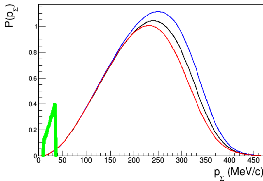
Fig. 1. (Colour on-line) Momentum distribution of \Sigma^+ following K^- capture in-flight on carbon nuclei. The thick grey/green distribution represents the Gamov peak. Other curves describe the dependence of the spectrum on the position of a 40 MeV wide resonance with E_r = 1410 MeV (red distribution), E_r = 1420 MeV (black distribution), T \equiv 1 (blue distributions) (from bottom to top). Normalisations are arbitrary, as only profiles are measured.
