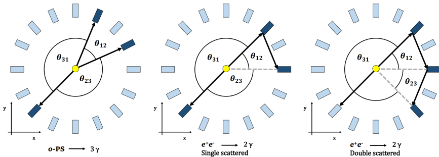
Fig. 1. Colour on-line) Definition of angles in XY view between registered gamma quanta with indexing fulfilling the condition \theta_{12} \leq \theta_{23} \leq \theta_{13} . Light rectangles represent scintillators, dark rectangles — scintillators with registered hit and yellow circle in the middle — annihilation region.
